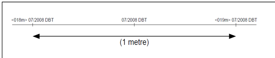
Figure 1: Cable Marking
