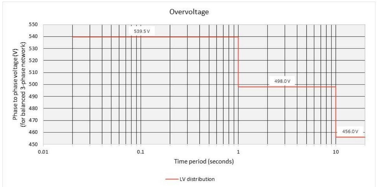
Figure 2.2 - Overvoltage Envelope – Low Voltage Distribution System
